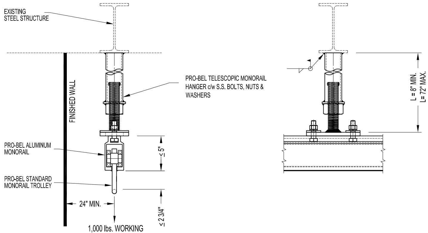
MNH350-7200: PRO-BEL MONORAIL HANGER BRACKET ASSEMBLY TYPE 3 - (WELD TO STEEL STRUCTURE)
