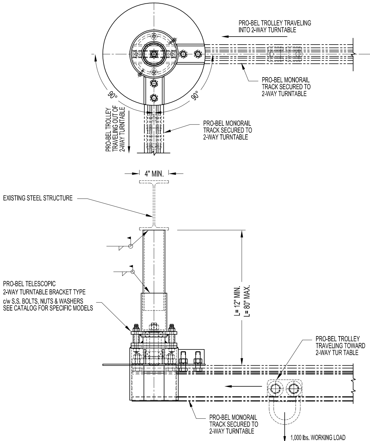
MN-TT250-8000: PRO-BEL 2-WAY TURNTABLE BRACKET ASS'Y (WELD TO STEEL STRUCTURE)
