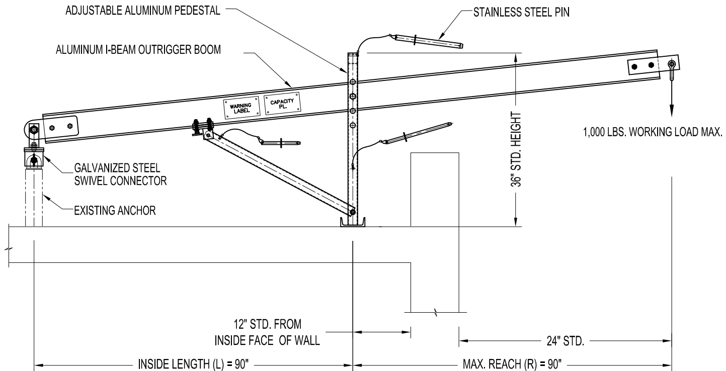
A-OR-0A21-090: PORTABLE OUTRIGGER PINNED TO ANCHOR w/ ADJUSTABLE PEDESTAL (TILTED)
