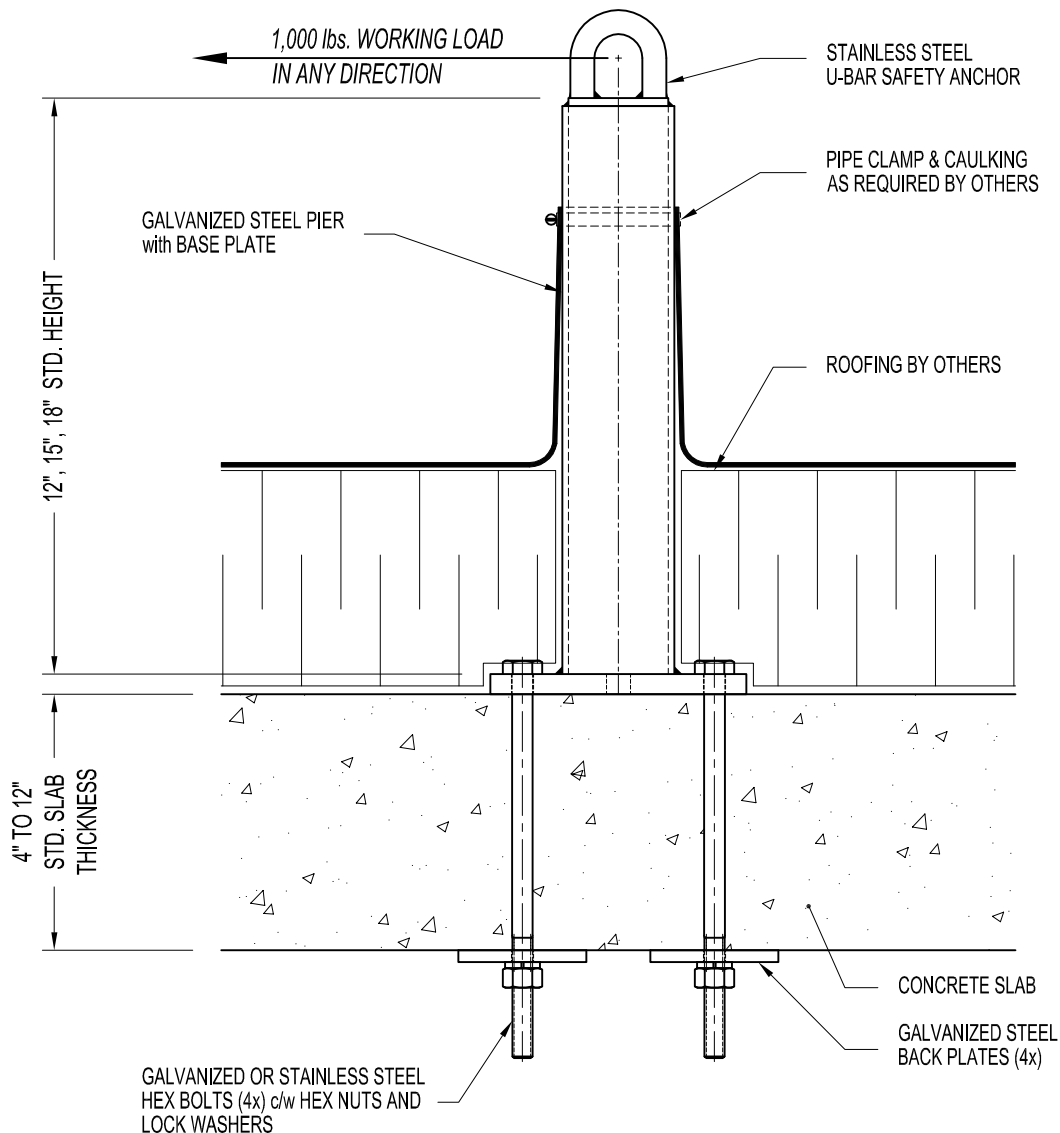
PBE73-00A4: THROUGH BOLTED ROOF ANCHOR (FOUR STUDS)
