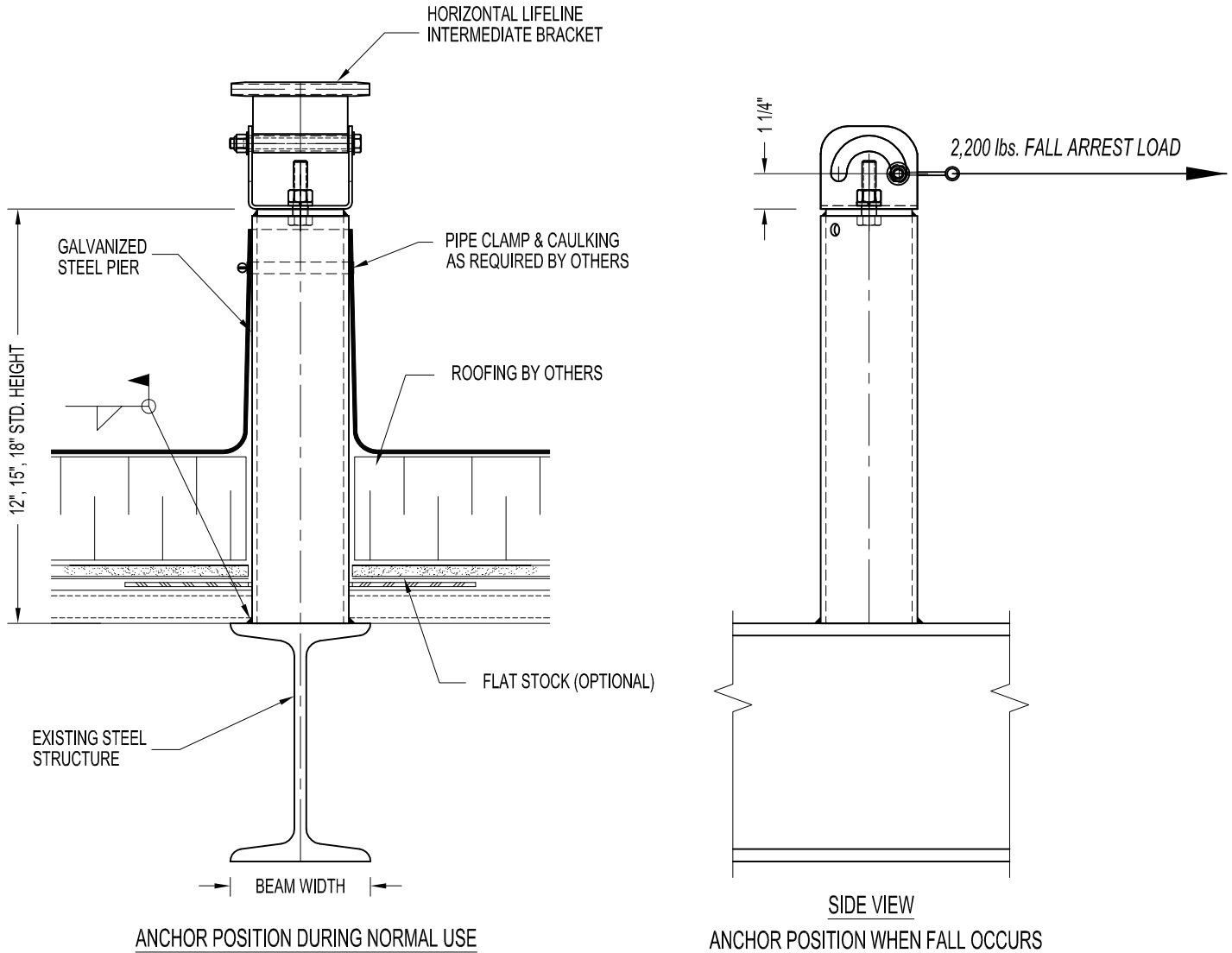
HLL-75IN1-0000: WELD TO STRUCTURE HLL INTERMEDIATE ANCHOR
