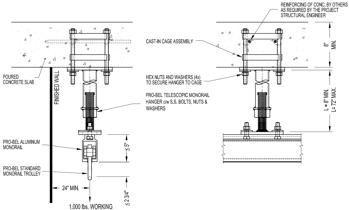
MNH330-7200: PRO-BEL MONORAIL HANGER BRACKET ASSEMBLY TYPE 3 - (CAST-IN CAGE)
